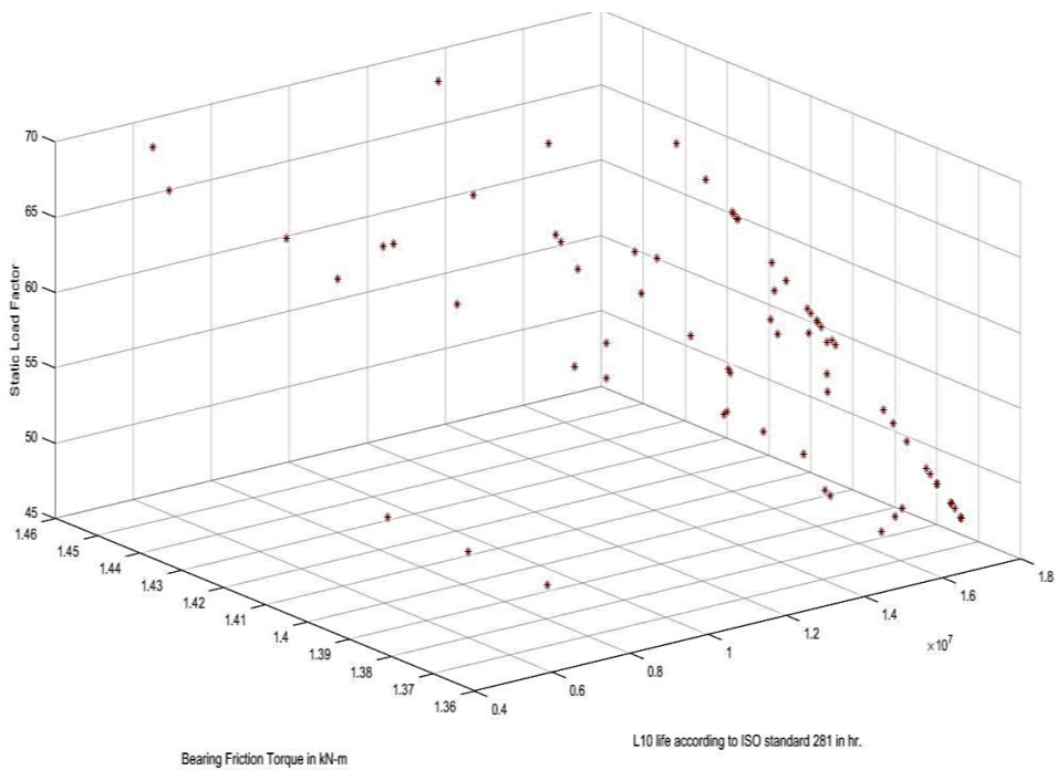
Figure 9: Pareto Front Attained by MOJAYAA for 45° Contact Angle
