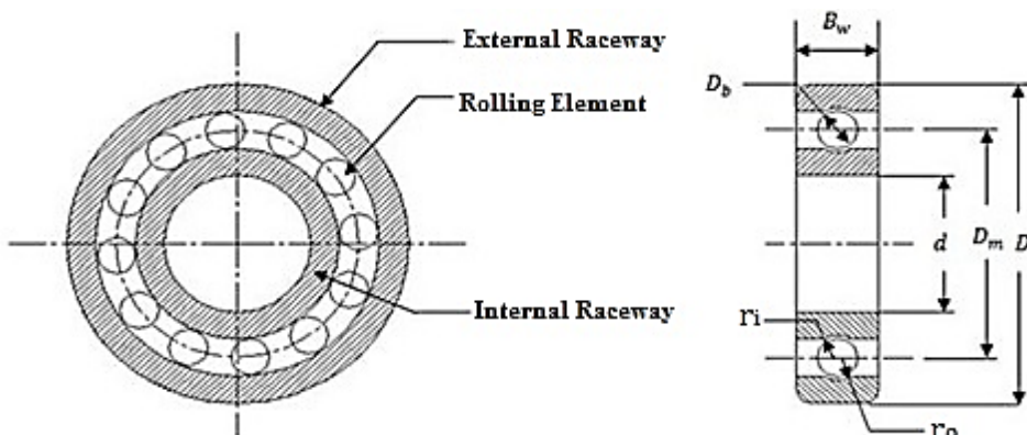
Figure 6: Rolling Bearing Design
