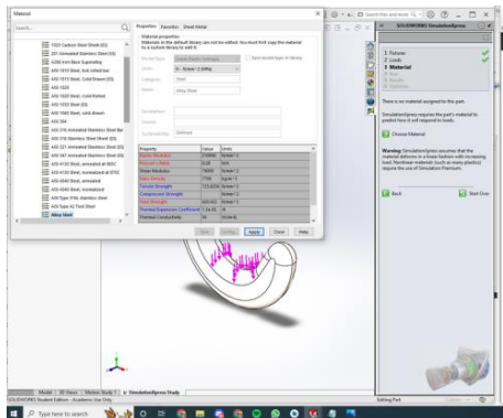
Figure 12. Selecting Material.
