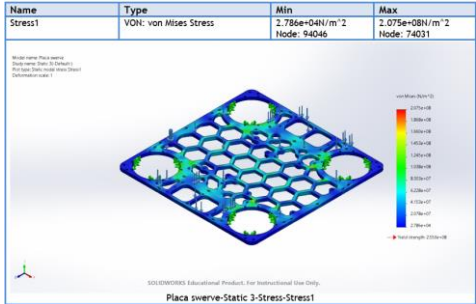
Figure 17. Von Misses stress graph for the main plate.
