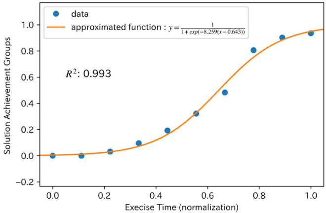
Figure 6. Example of fitting to a sigmoid function
